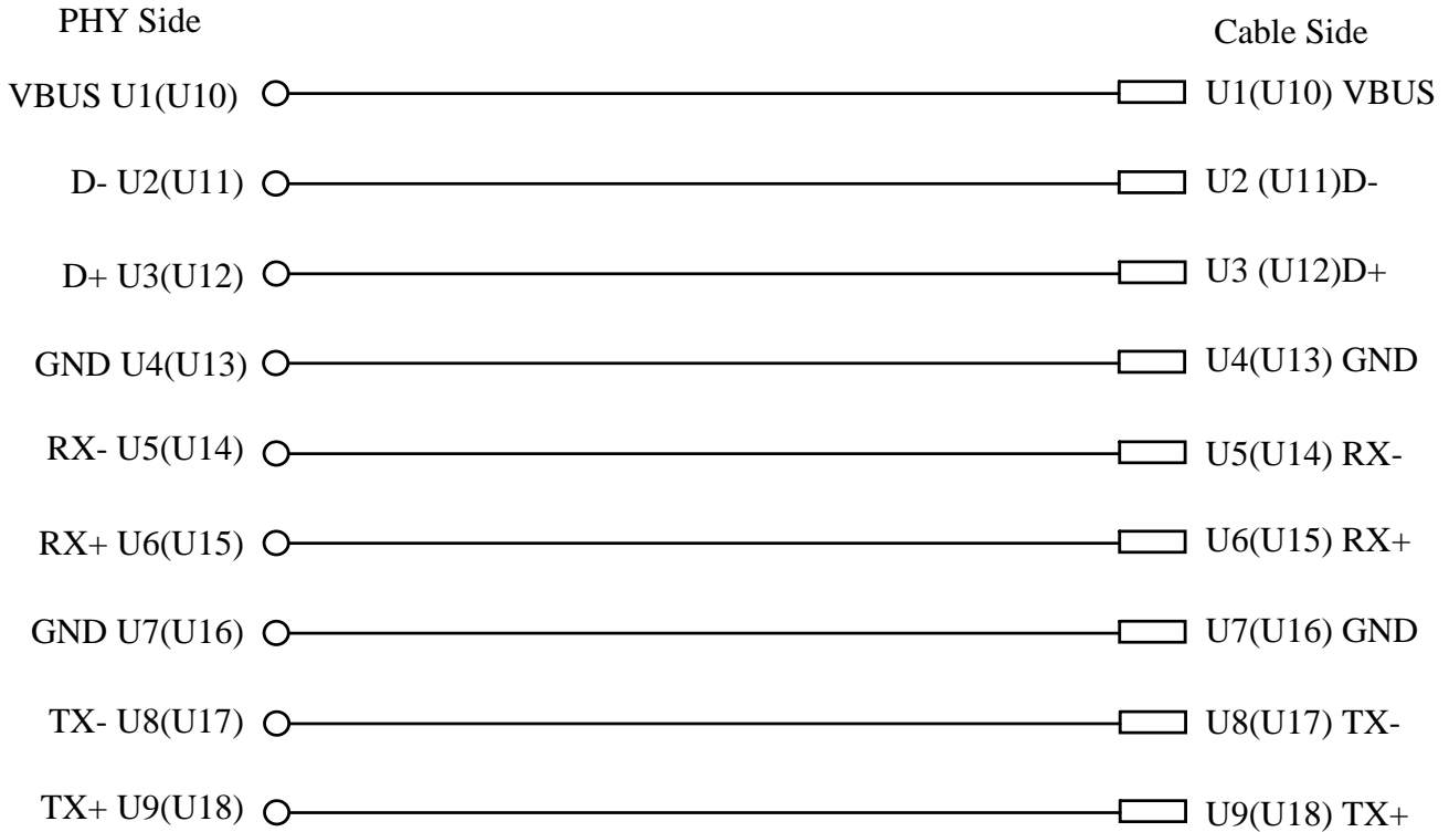
USB 3.2 GEN 1 Standard-A connector Pin Assignment
