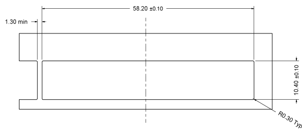
PANELCUTOFF FOR BELLY TO BELLY MOUNTING (SPRING FINGERS)
