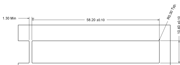
PANELCUTOFF FOR SINGLE SIDE MOUNTING (SPRING FINGERS)
