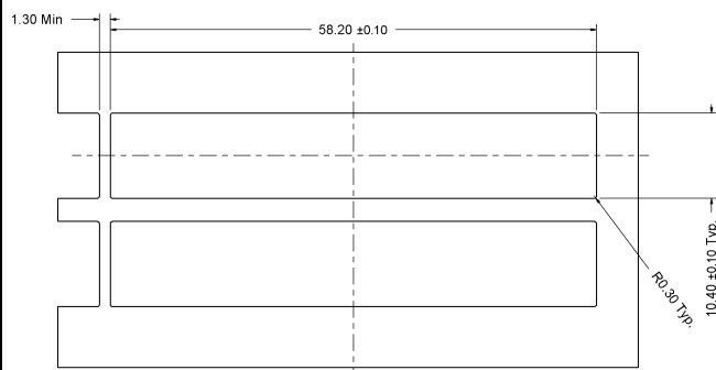
PANELCUTOFF FOR BELLY TO BELLY MOUNTING (SPRING FINGERS)
