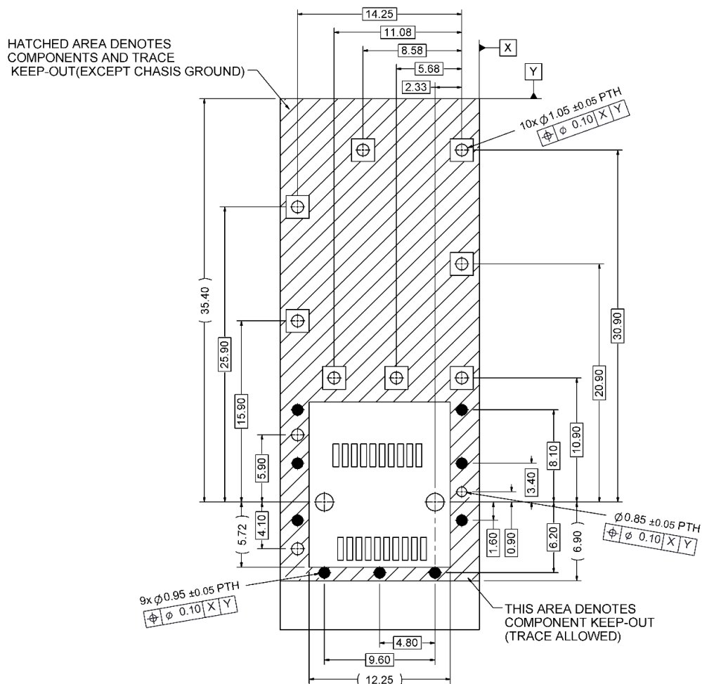
PCB LAYOUT FOR SINGLE SIDE MOUNTING
