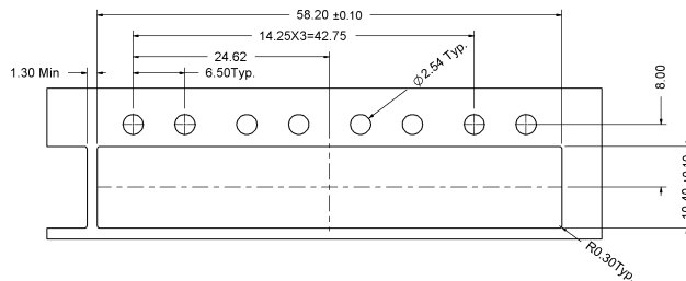
PANELCUTOFF FOR BELLY TO BELLY MOUNTING(SPRING FINGERS)
