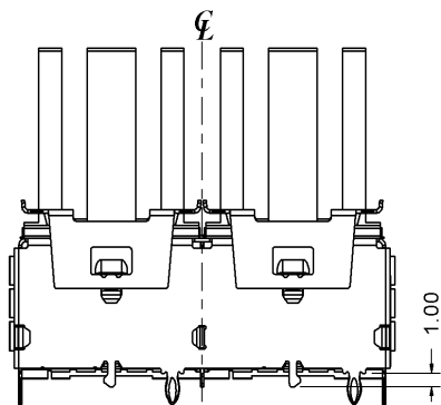
RIGHT VIEW
