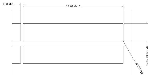
PANELCUTOFF FOR BELLY TO BELLY MOUNTING(SPRING FINGERS)
