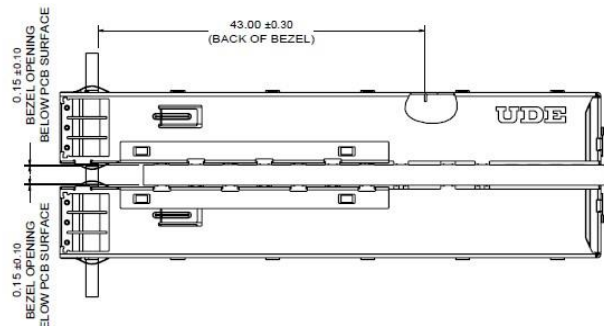
PANELCUTOFF FOR BELLY TO BELLY MOUNTING(SPRING FINGERS)
