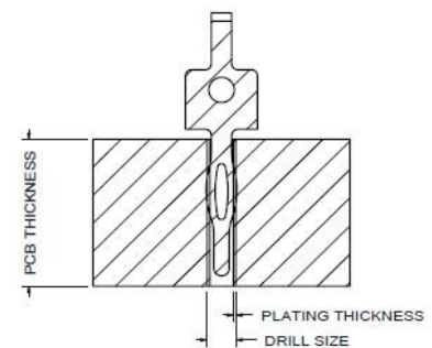
RECOMMENDED MOTHER BOARD THROUGH HOLE DIMENSION
