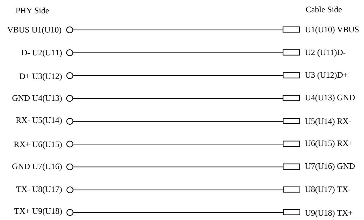
USB 3.2 GEN 2 Standard-A connector Pin Assignment
