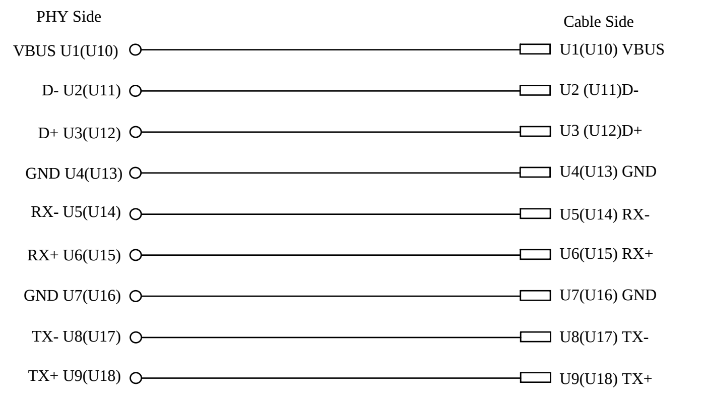
USB 3.2 GEN 1 Standard-A connector Pin Assignment
