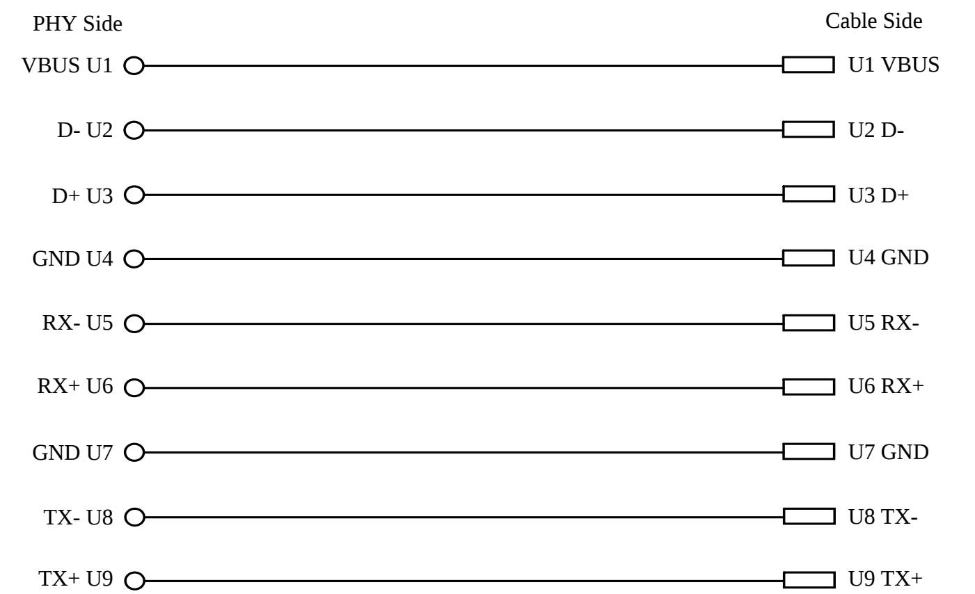
USB 3.2 GEN 2 Standard-A connector Pin Assignment
