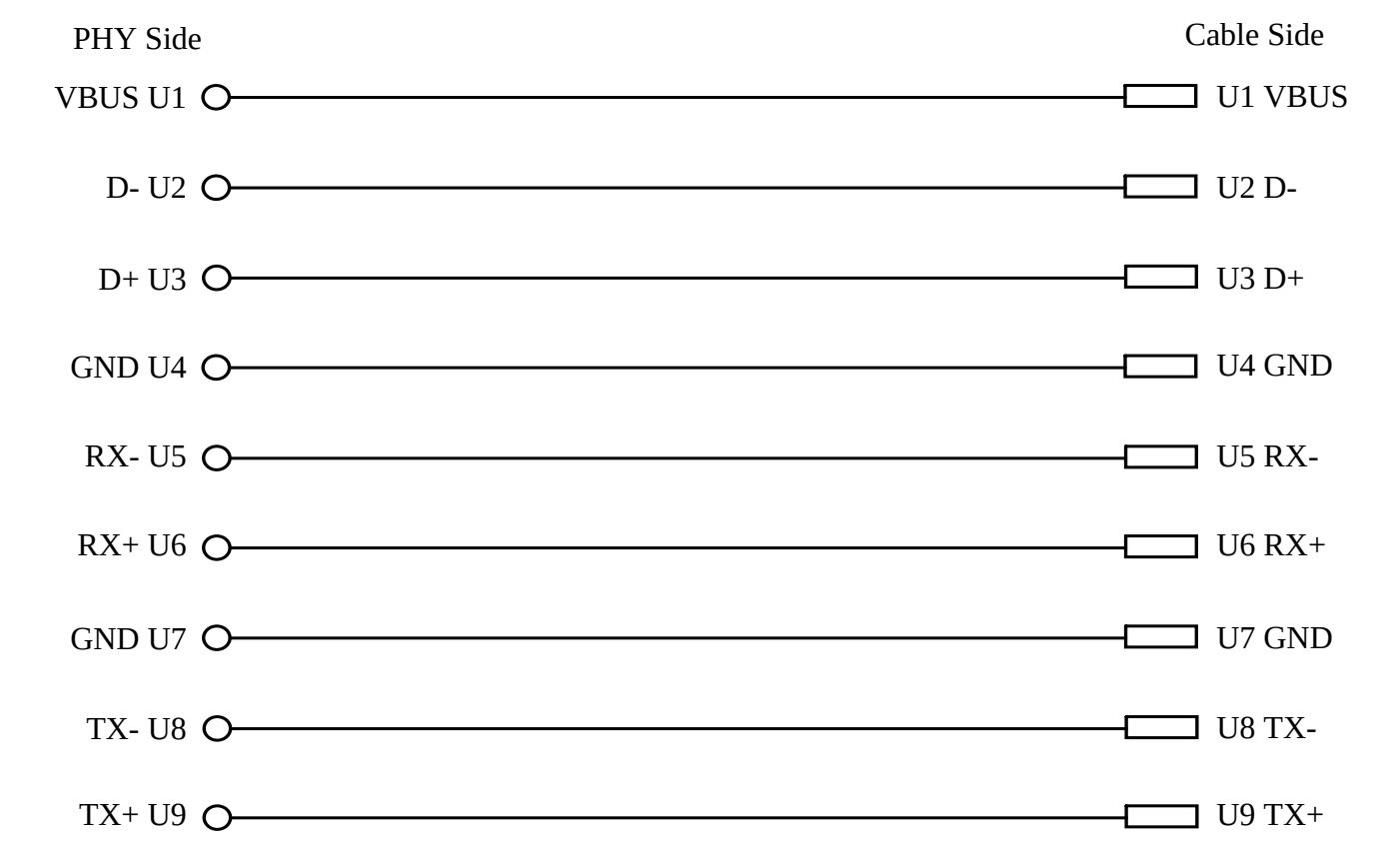
USB 3.2 GEN 1 Standard-A connector Pin Assignment
