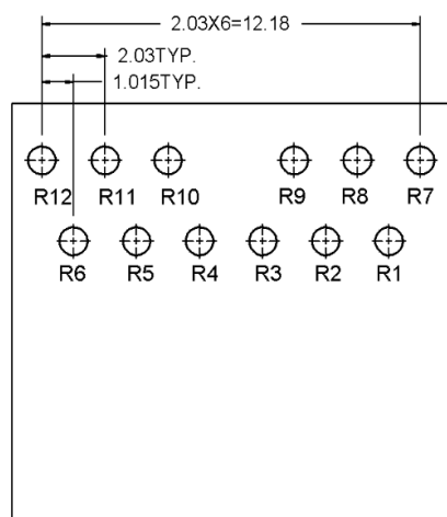
Detail D
